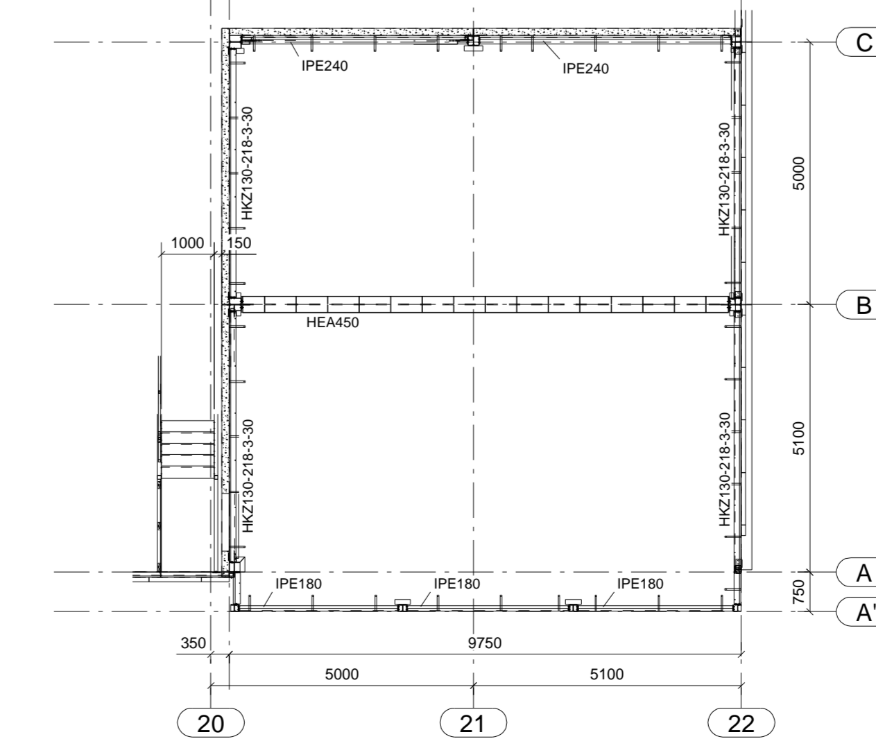
TUSSENVLOER +3.020 (B.K.S)
