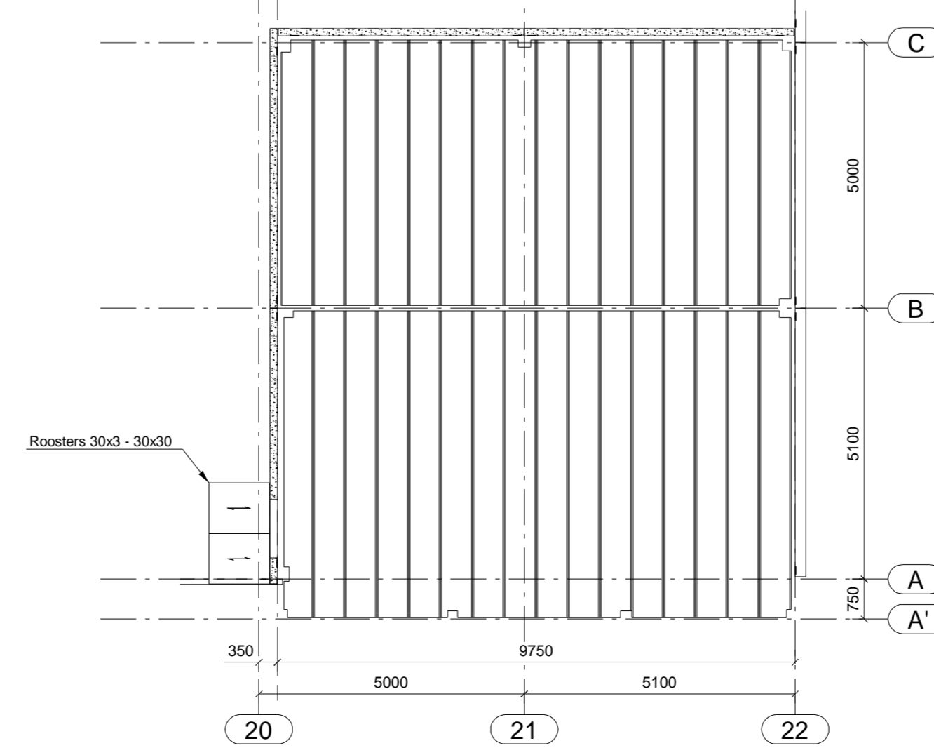
TUSSENVLOER +3.020 (B.K.S)
