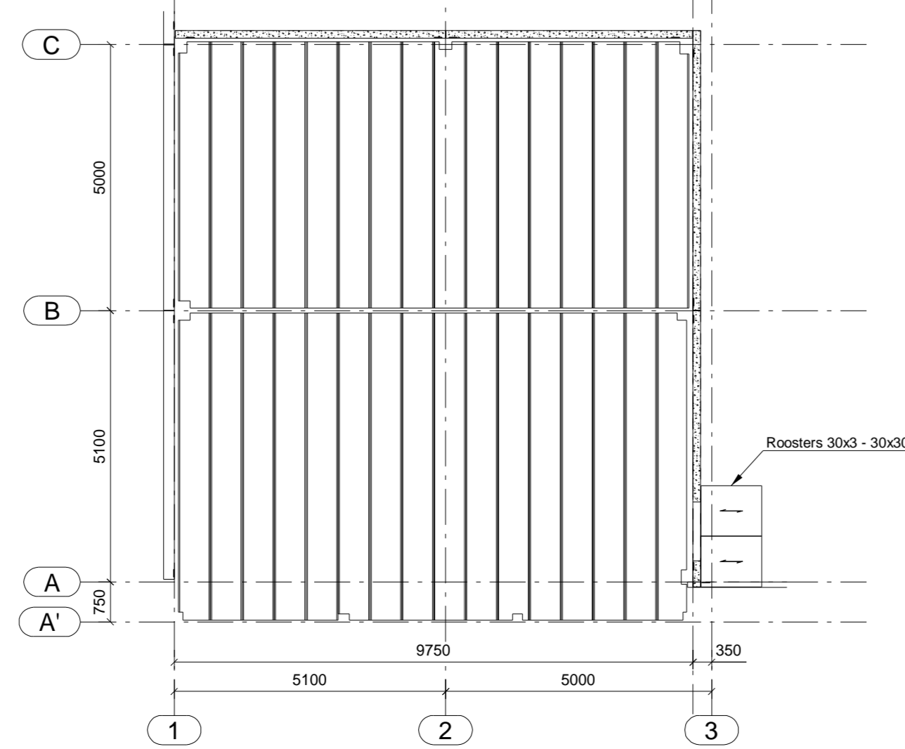
TUSSENVLOER +3.020 (B.K.S)
