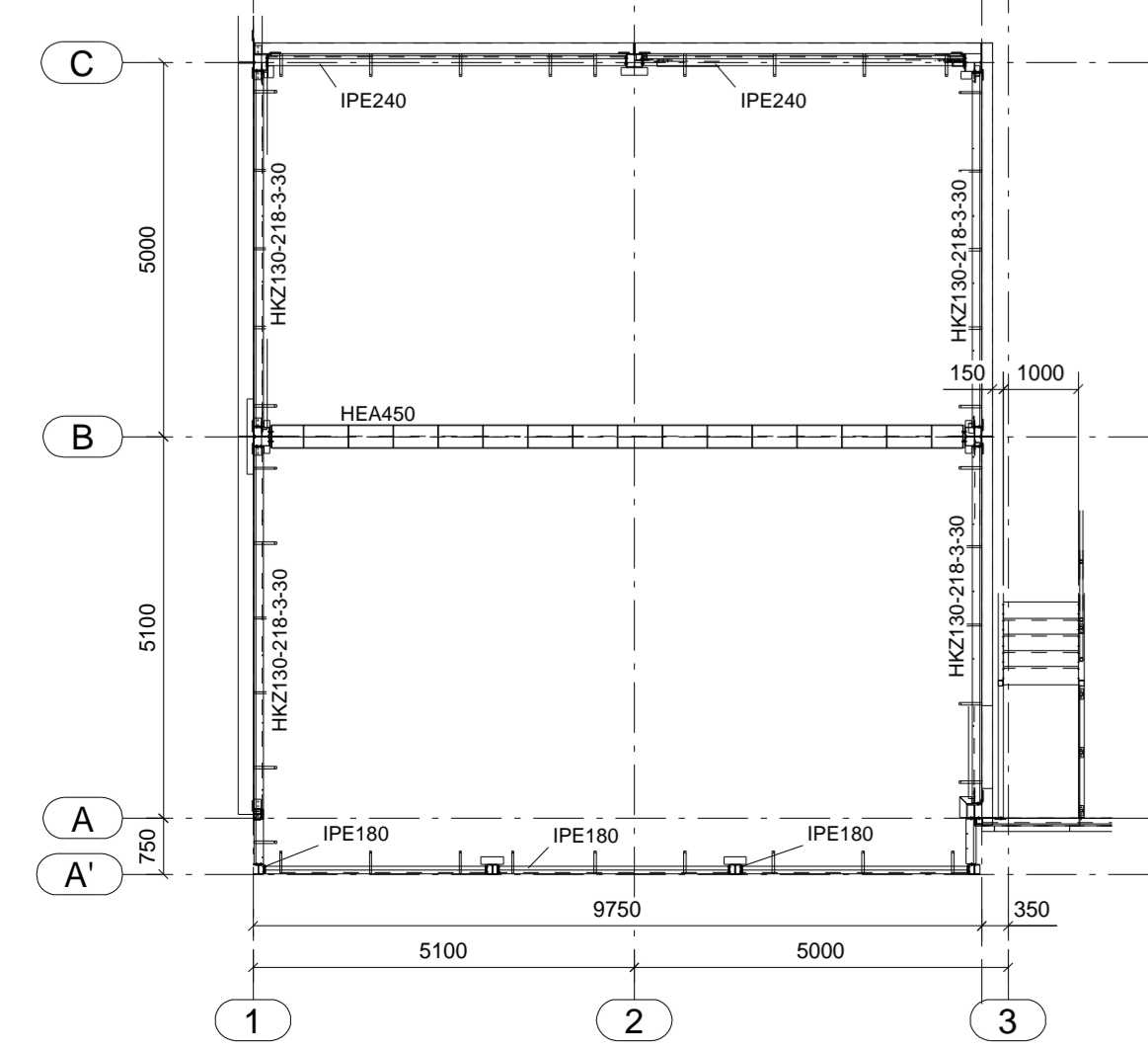
TUSSENVLOER +3.020 (B.K.S)
