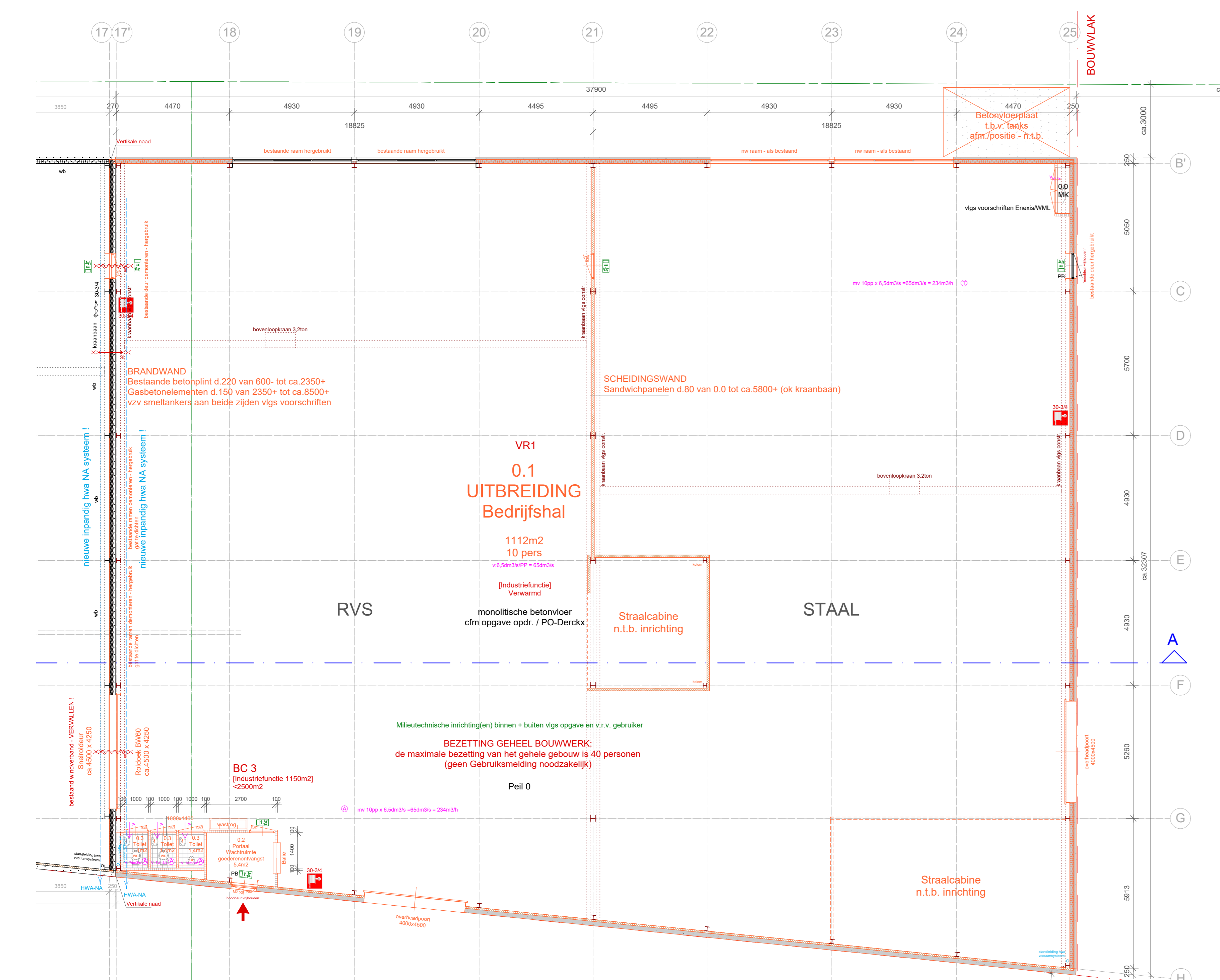
Begane Grond [peil] BOUWPEIL = reeds bestaand peil 0
